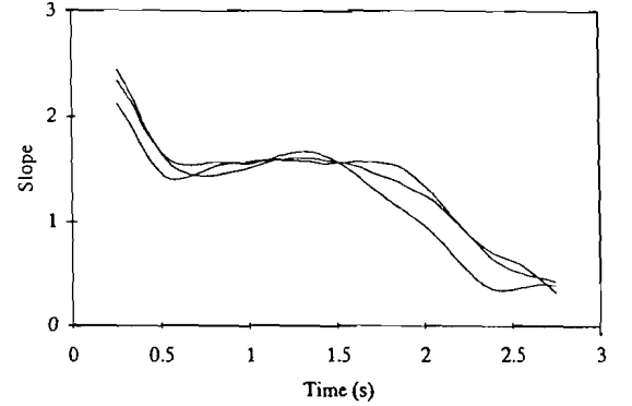
Fig. 10. Plot of (d/dt) \langle \ln d_j(i) \rangle versus i \Delta t using our algorithm with three 5000-point realizations of the Lorenz attractor.
