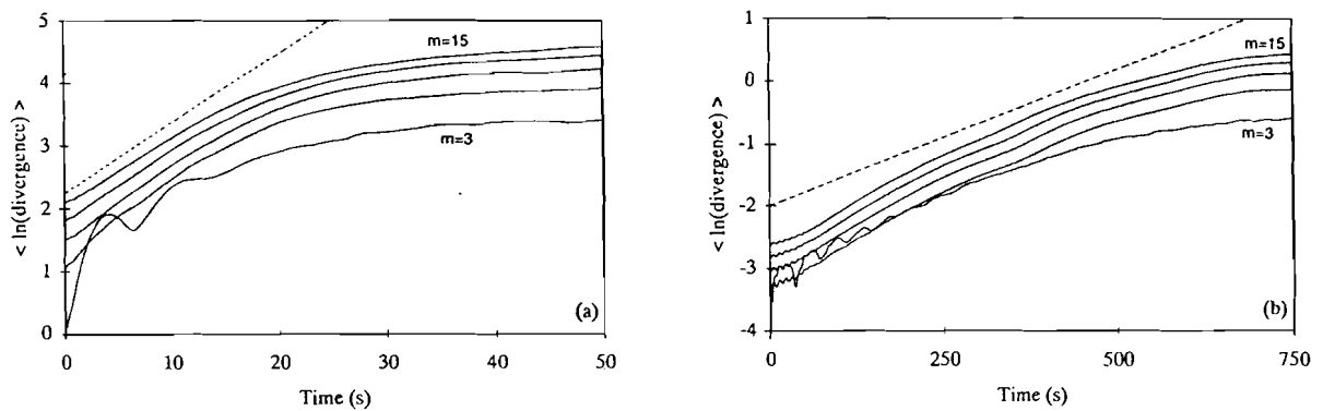
Fig. 8. Results for systems with two positive Lyapunov exponents. For each plot, the solid curves are the calculated results, and the slope of the dashed curve is the expected result. See table 7 for details. (a) Rössler-hyperchaos. (b) Mackey-Glass.
