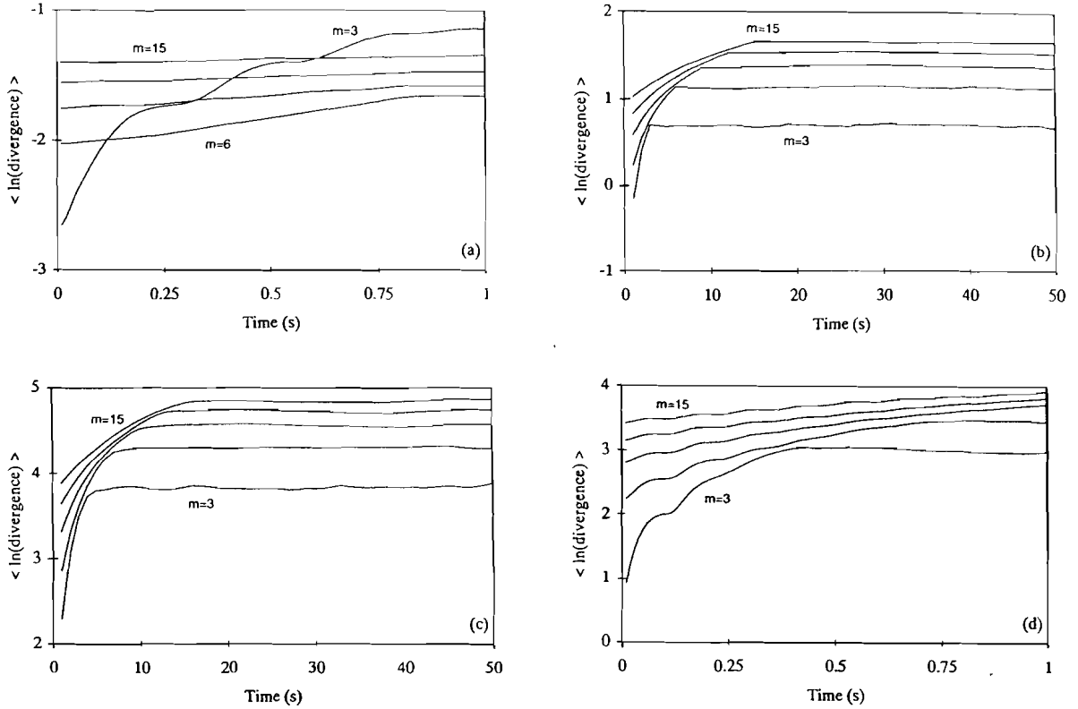
Fig. 9. Effects of embedding dimension for non-chaotic systems. (a) Two-torus. (b) White noise. (c) Bandlimited noise. (d) "Scrambled" Lorenz.
