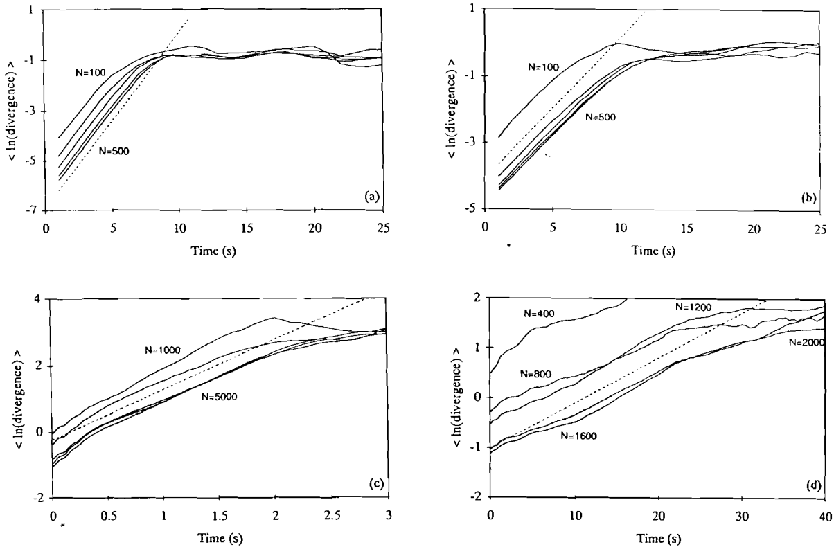
Fig. 4. Effects of time series lengths. For each plot, the solid curves are the calculated results, and the slope of the dashed curve is the expected result. See table 3 for details. (a) Logistic map. (b) Hénon attractor. (c) Lorenz attractor. (d) Rössler attractor.
