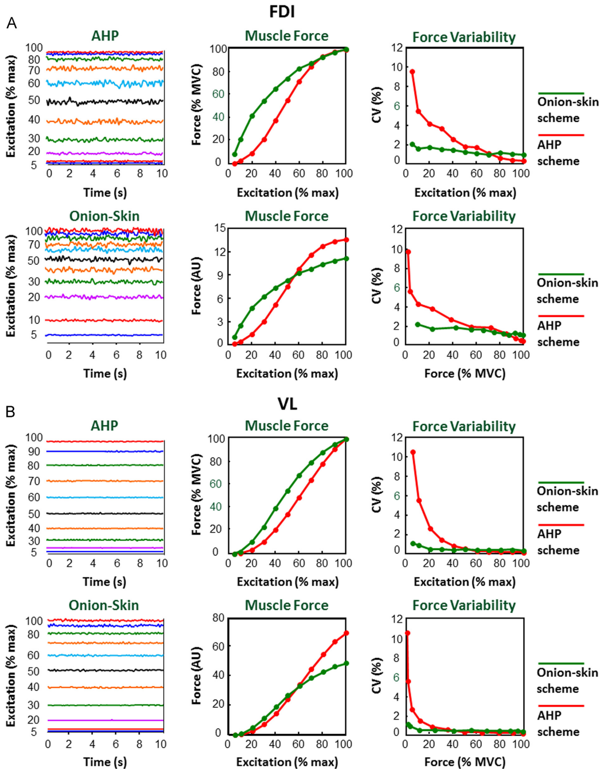
Fig. 4. Properties of the muscle force for the Onion-Skin and AHP schemes. (Left panels) A 10-s interval of the muscle force produced by the AHP (top) and Onion-Skin (bottom) schemes at increasing levels of input excitation (5, 10 to 100% in steps of 10% input excitation). (Middle panels) Average normalized muscle force (in % MVC, top) and absolute muscle force (in arbitrary unit (AU), bottom) generated by the Onion-Skin (green) and AHP (red) schemes at increasing levels of input excitation. (Right panels) Coefficient of variation (CV) of the muscle force produced by the Onion-Skin (green) and AHP (red) schemes at increasing levels of input excitation (top) and muscle force (bottom). Results from the FDI and VL muscles are presented in panels A and B, respectively. (For interpretation of the references to color in this figure legend, the reader is referred to the web version of this article.)
