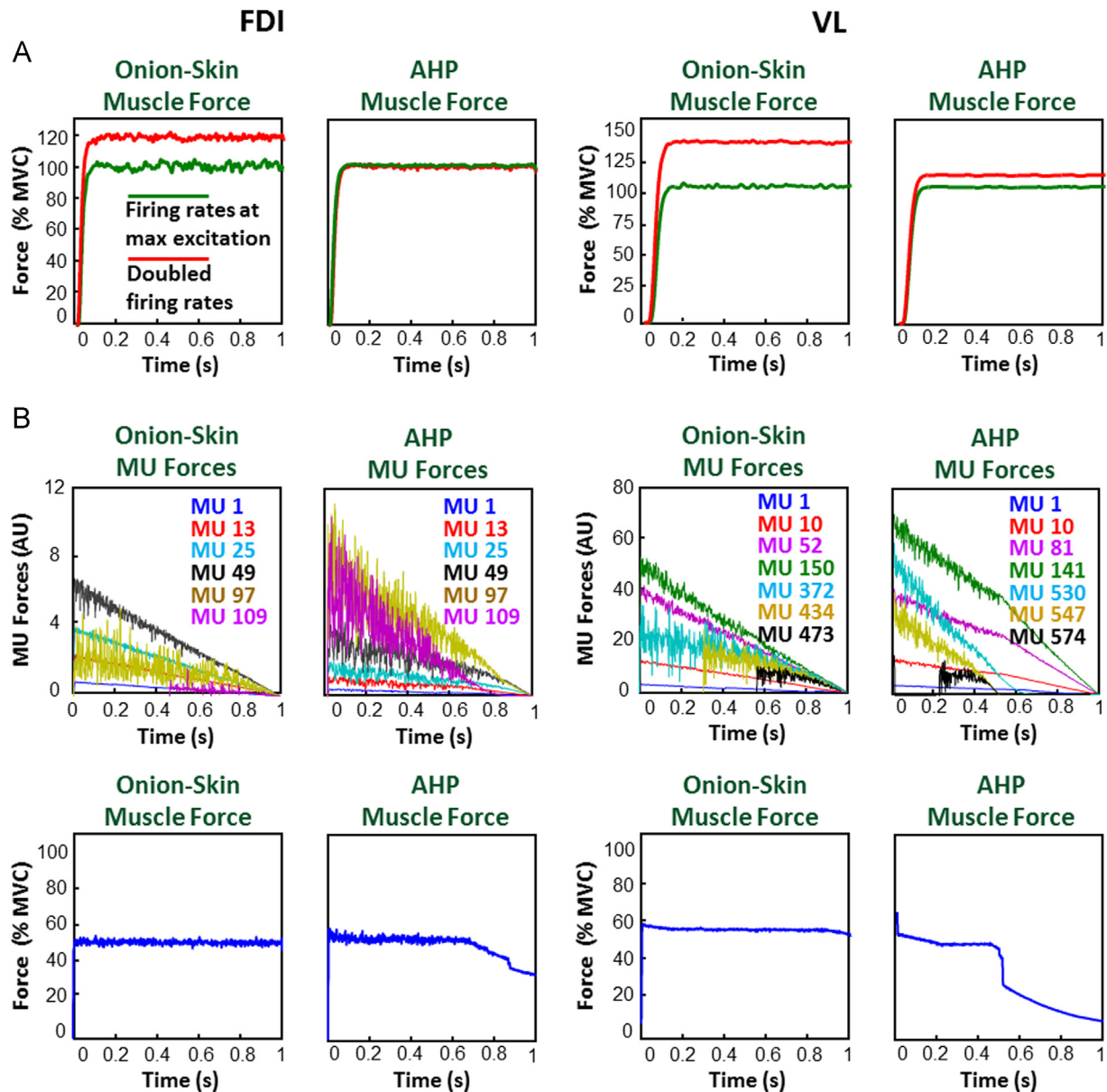
Fig. 5. Maximal force generation capacity and endurance time for the Onion-Skin and AHP schemes. (A) Output muscle force for the Onion-Skin and AHP schemes when motor unit firing rates are doubled (red) from their value at maximal input excitation (green) in the FDI (left) and VL (right) muscles. (B) Time-dependent motor unit (MU) force (top) and muscle force (bottom) force for the Onion-Skin and AHP schemes in the FDI (left) and VL (right) muscles. Six and seven motor units are shown for clarity in the FDI and VL, respectively. The amplitude of the motor unit force twitches decrease as a function of time, firing rate and recruitment threshold determining different time-varying patterns in the individual MU forces. (For interpretation of the references to color in this figure legend, the reader is referred to the web version of this article.)
