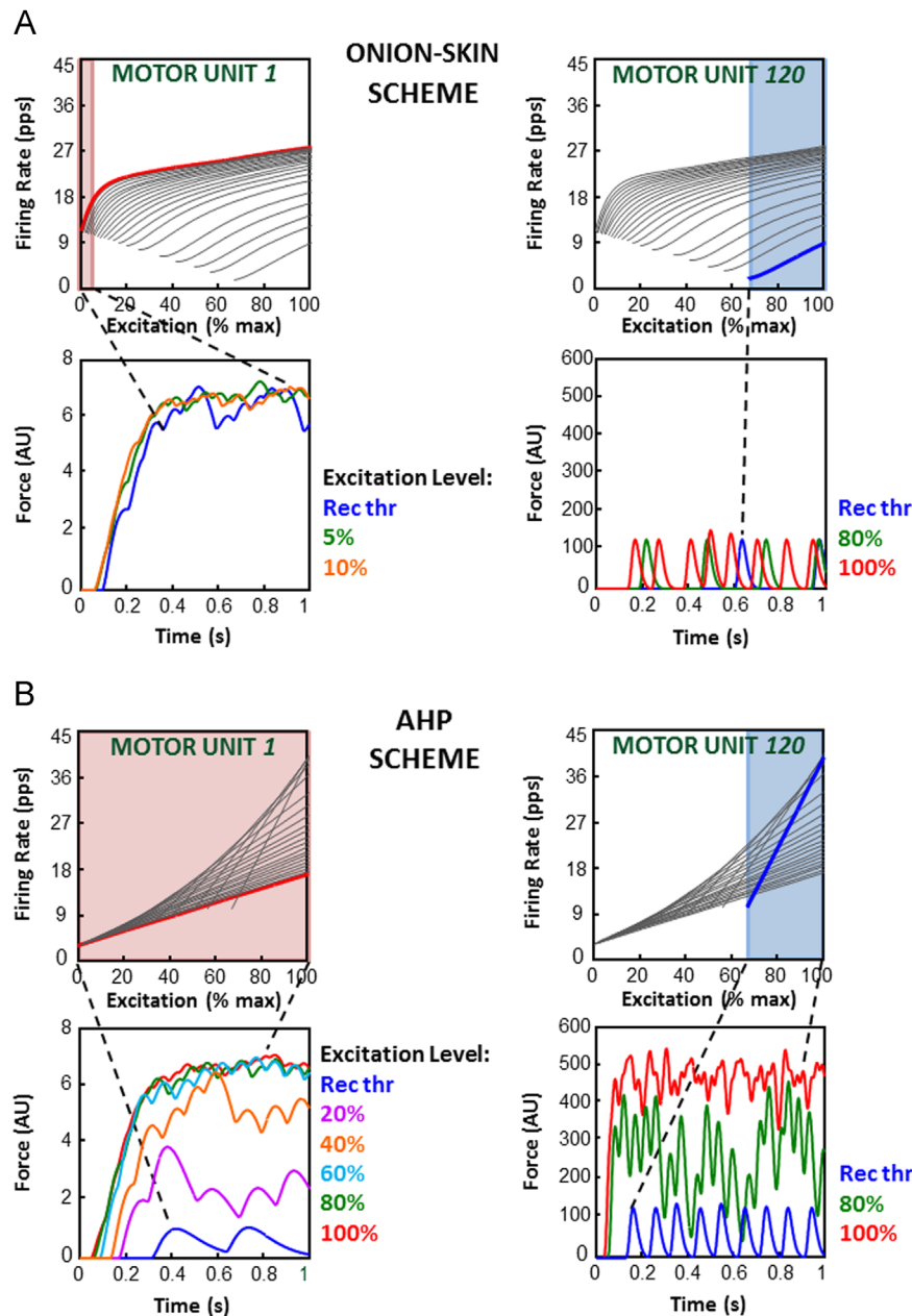
Fig. 2. Low and high-threshold motor unit forces for the Onion-Skin and AHP schemes in the FDI. (A and B, bottom panels) Force produced by the first (#1 on the left) and the last (#120 on the right) recruited motor units at increasing input excitation values starting from that at recruitment (Rec Thr). Fully fused force is achieved at maximal input excitation in the AHP scheme (B) for both motor units. It is achieved at low input excitation for motor unit #1, but not for motor unit #120, in the Onion-Skin scheme (A). (A and B, top panels) The firing rate trajectories of motor units #1 and #120 are highlighted in the firing rate spectra of the Onion-Skin (A) and AHP (B) schemes. The input excitation range from recruitment to full force fusion, if achieved, is highlighted. (For interpretation of the references to color in this figure legend, the reader is referred to the web version of this article.)
